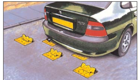
Flowplates can be installed as a single row across the roadway, or for maximum effect, as a staggered double row
